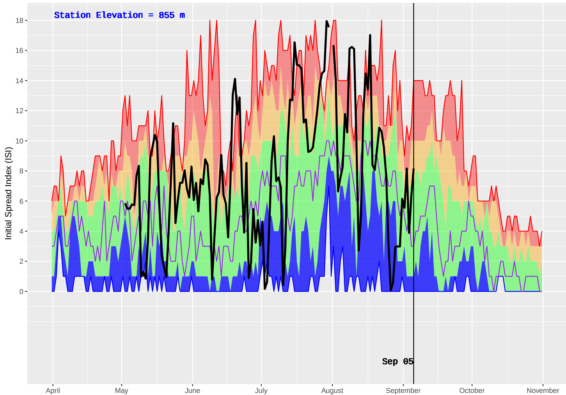
AUGUST LAKE (836) : Historical (2003–2016) and Current (2018) Daily Initial Spread Index (ISI)
