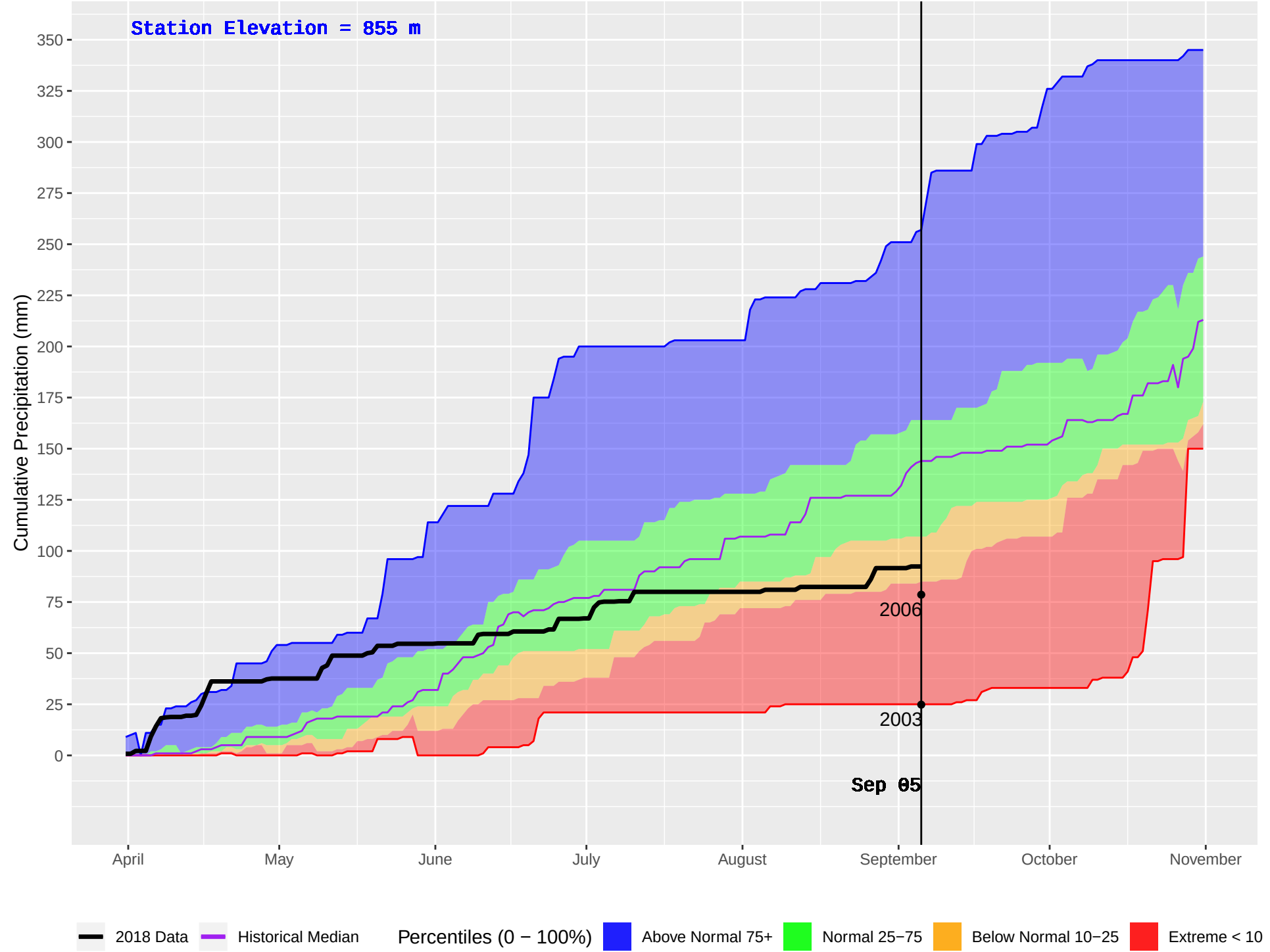
AUGUST LAKE (836) : Historical (2003–2016) and Current (2018) Daily Cumulative Precipitation
