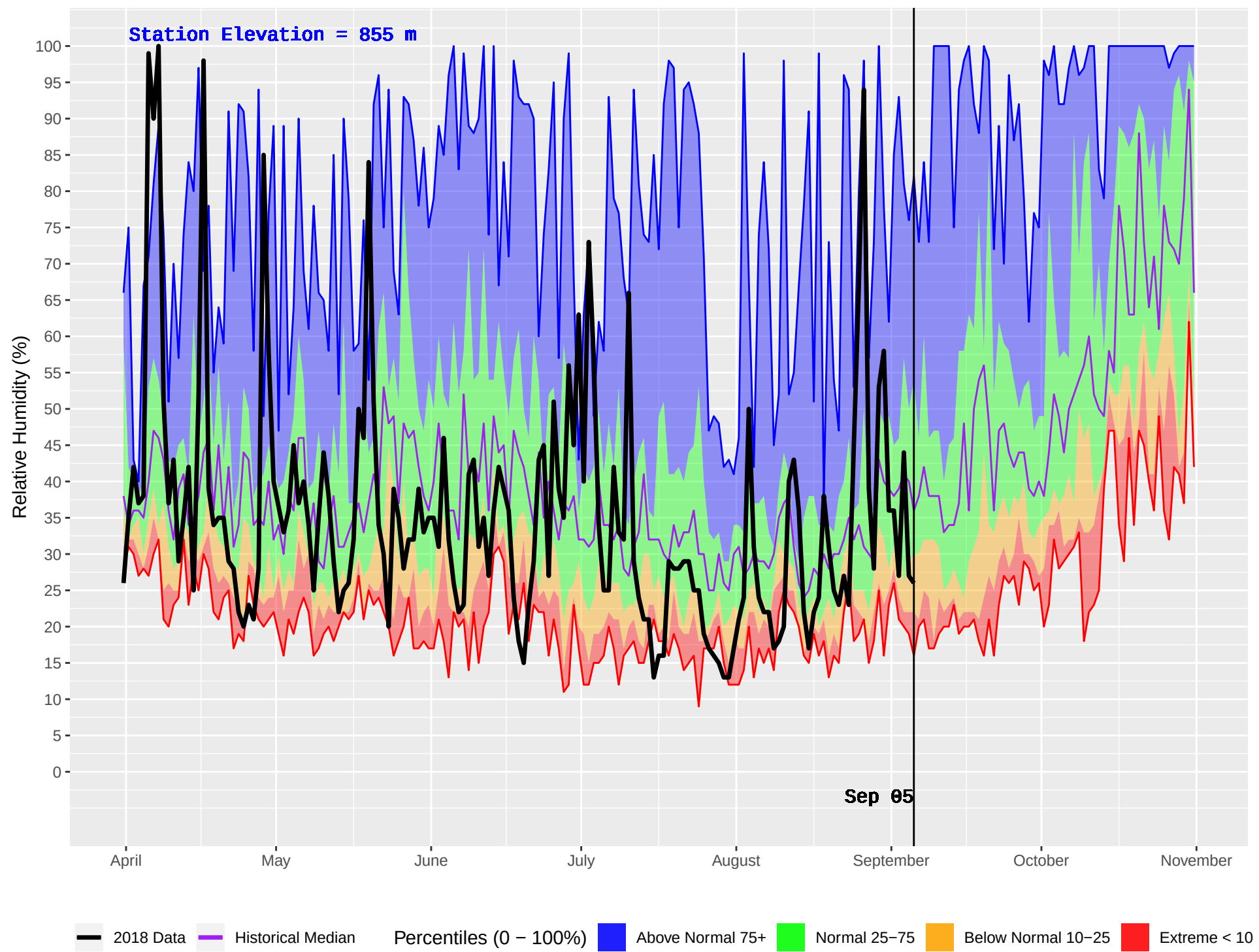
AUGUST LAKE (836) : Historical (2003–2016) and Current (2018) Daily Relative Humidity
