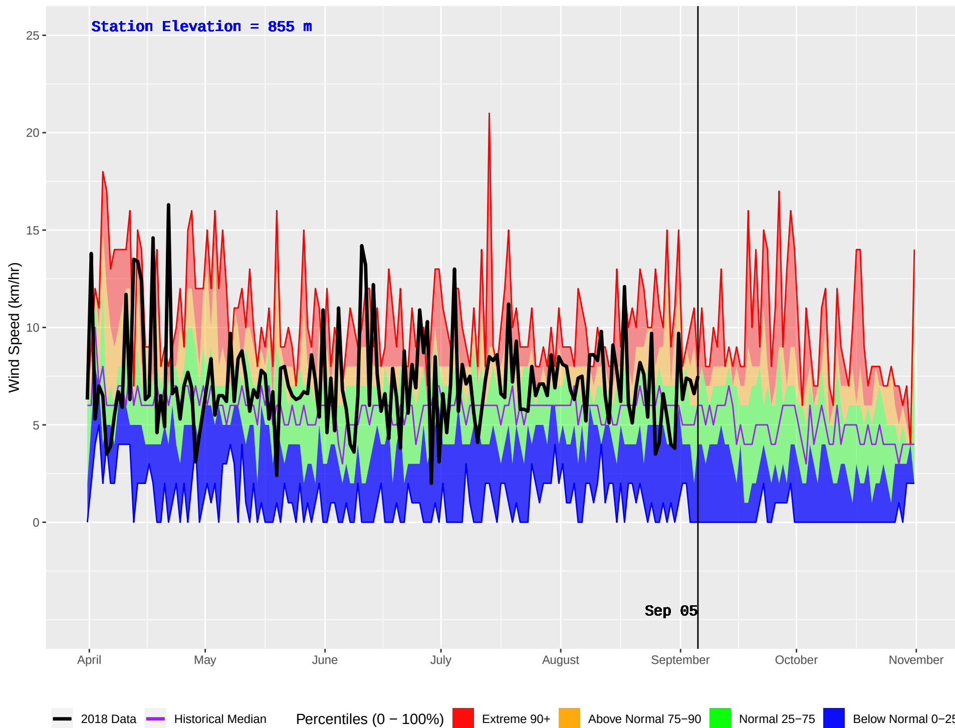
AUGUST LAKE (836) : Historical (2003–2016) and Current (2018) Daily Wind Speed
